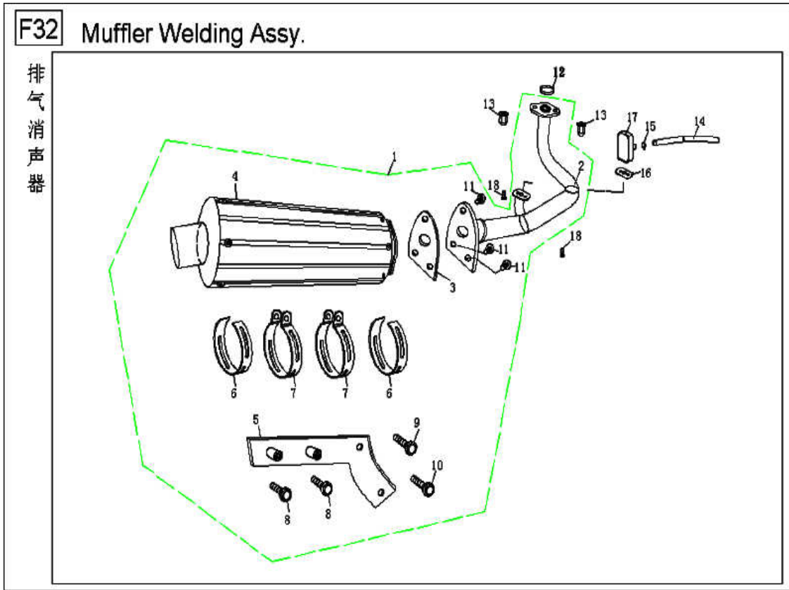
F32 Muffler welding assy.
