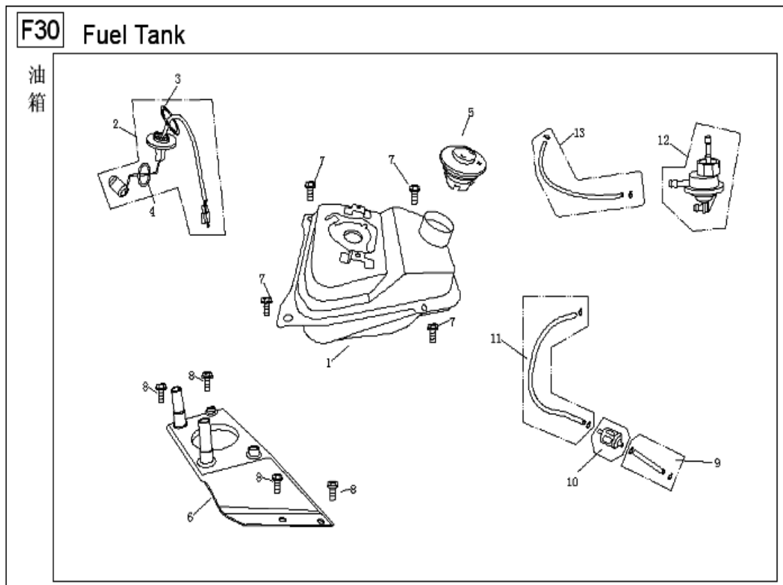
F30 Fuel tank
