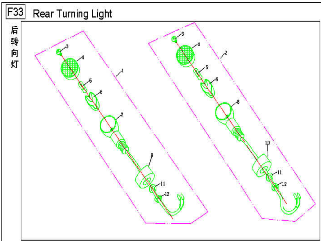
F33 Rear turning light.
