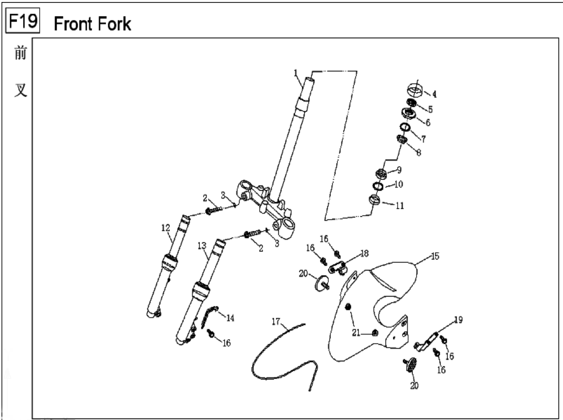
F19 Front fork
