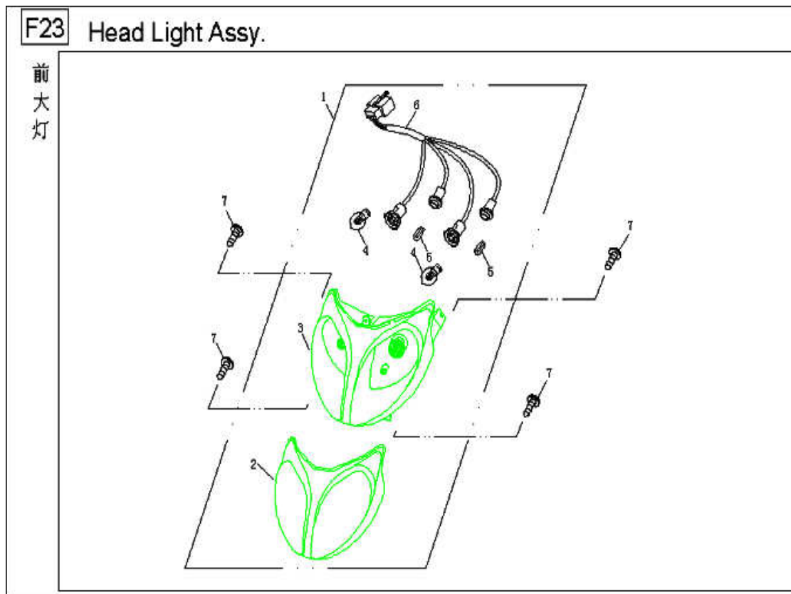
F23 Head light assy
