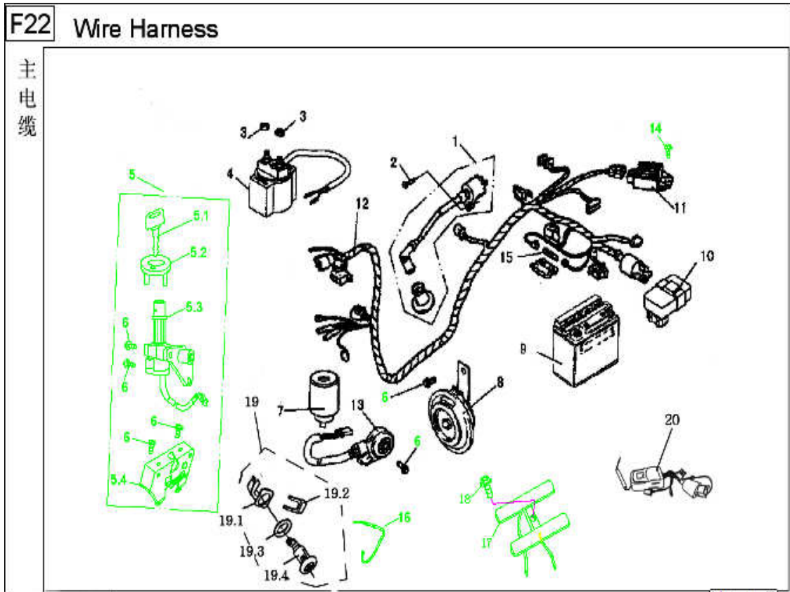
F22 Wire harness
